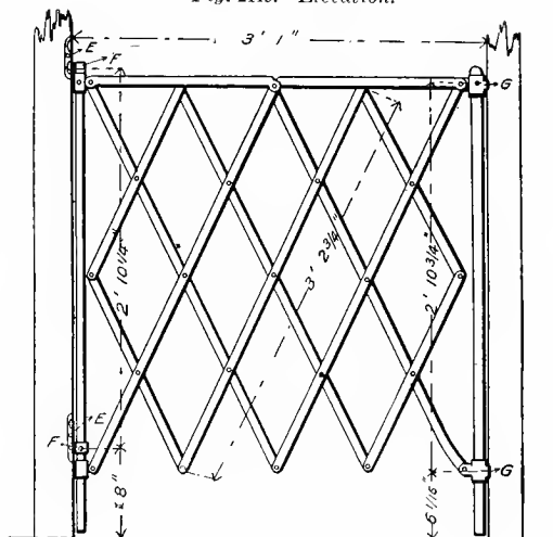
Fig. 2449. Elevation.
